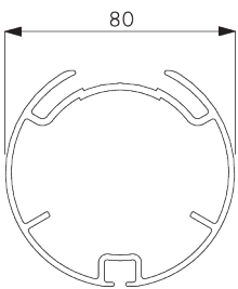
SG 4901 Tube ø 80 mm
