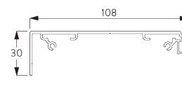
SG 11530 Installation profile fascia 110 mm
