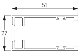
SG 11542 Side guide channel
