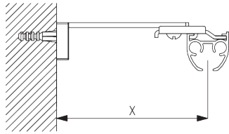
Square Smart Fix SG 11210 - SG 11215 and bracket SG 3832:
